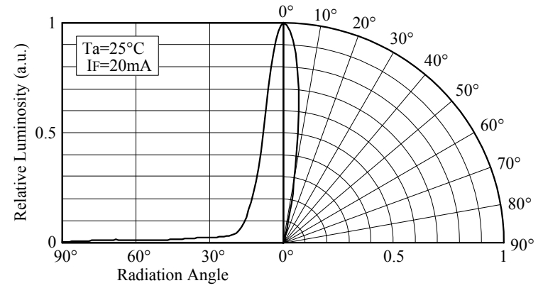
■ Directivity (NSPB500(S))
